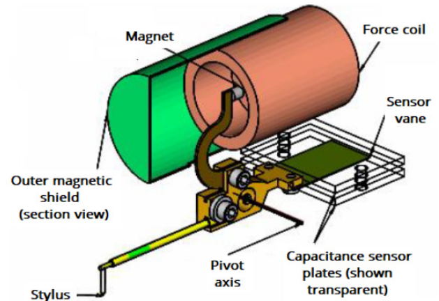
Figure 4. Tencor P-Series and HRP-Series LVDC sensor schematic.
