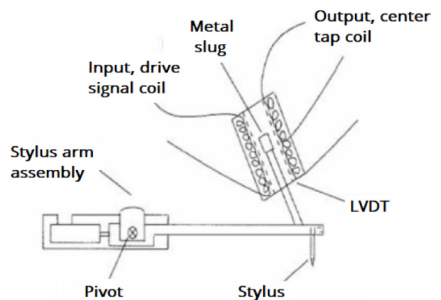
Figure 2. Alpha-Step IQ sensor schematic.
